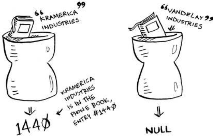
Looking for companies in a phone book with binary search
