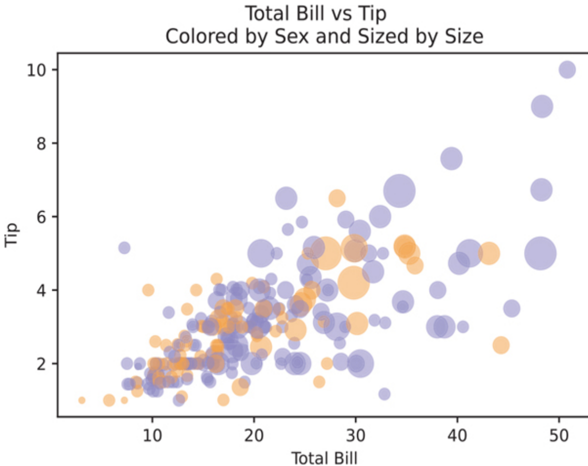
Figure 3.11 Matplotlib scatter plot with sex for the point color and size as point size
