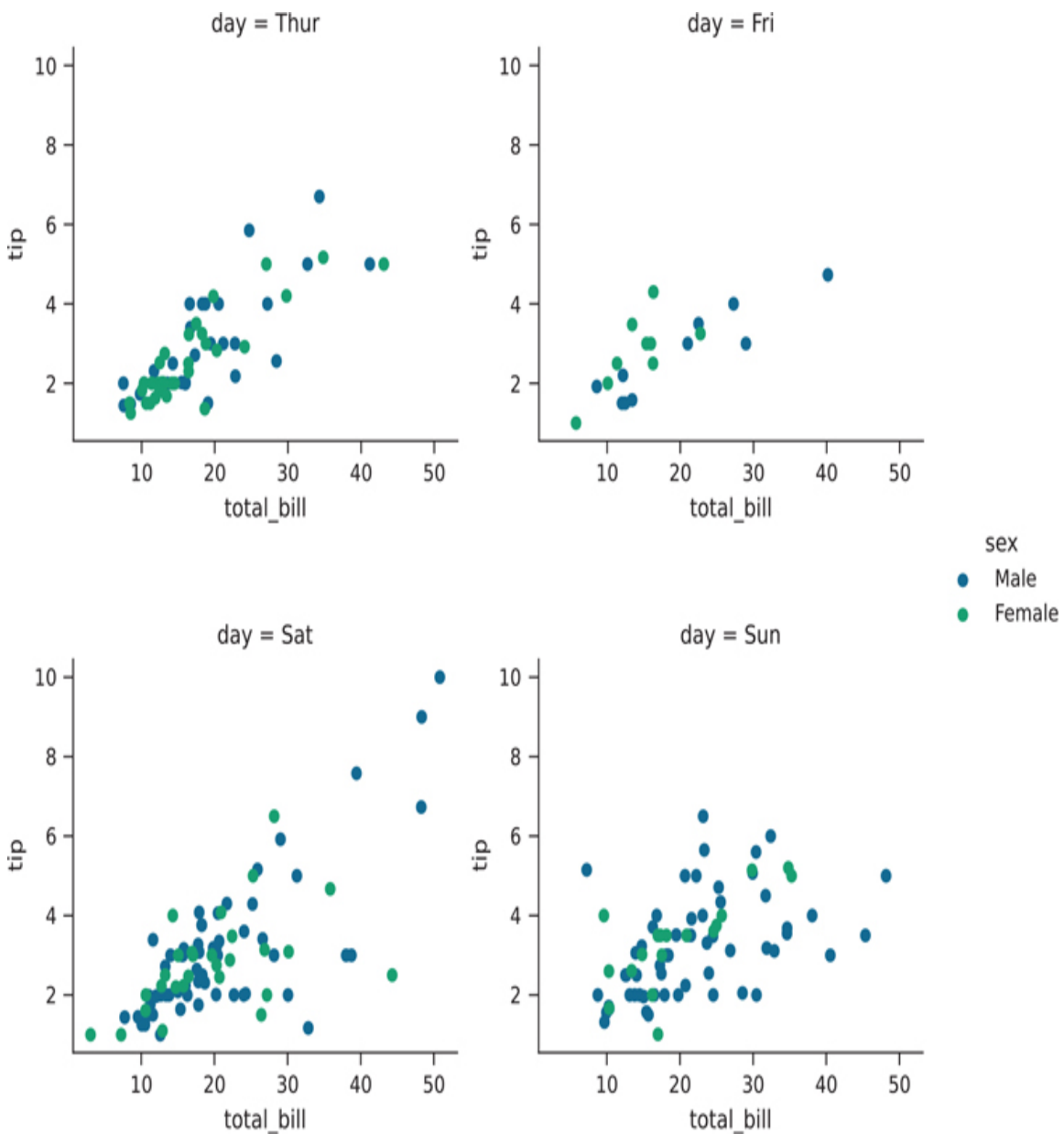
Figure 3.37 Seaborn plot with manually created facets that contain multiple variables
