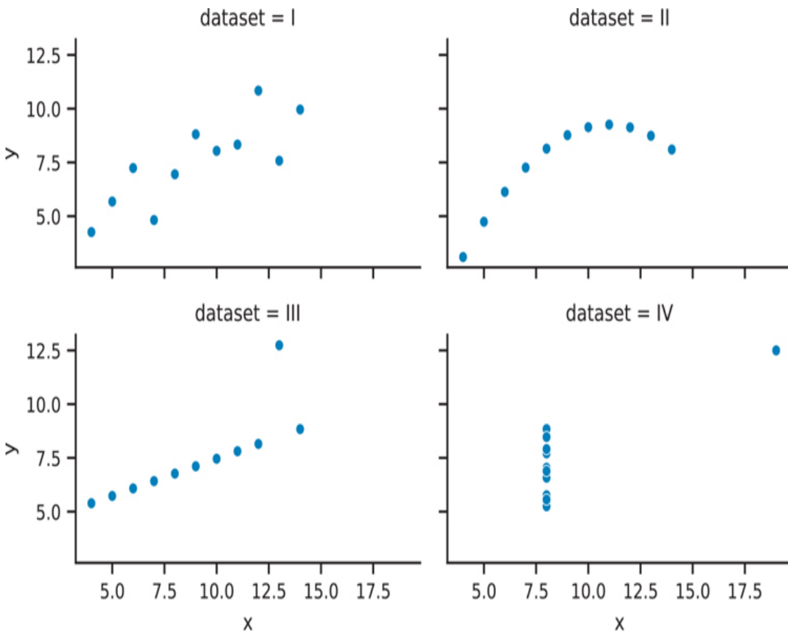
Figure 3.34 Seaborn Anscombe plot with facets
