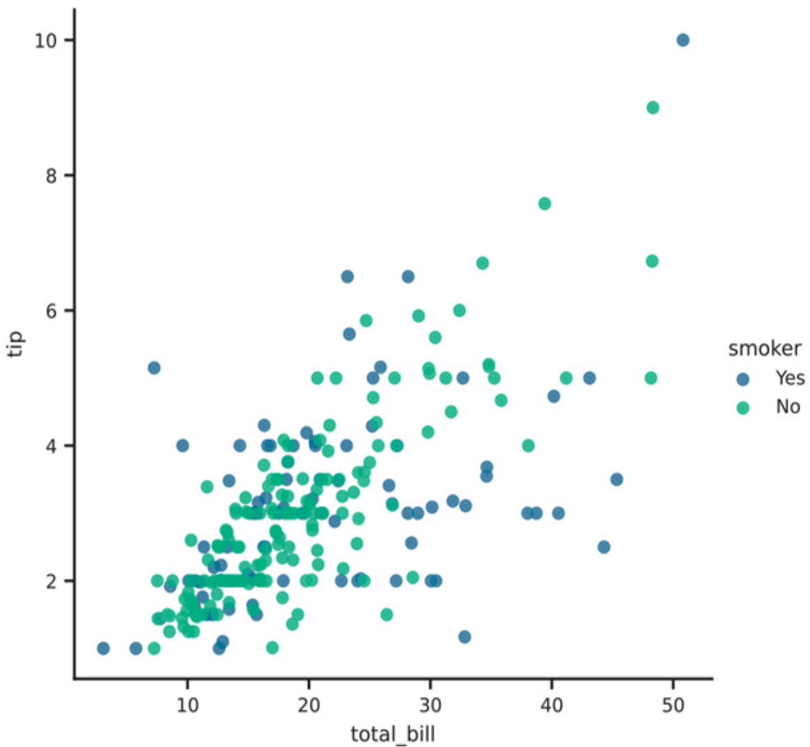
Figure 3.31 Seaborn lmplot plot with hue parameter
