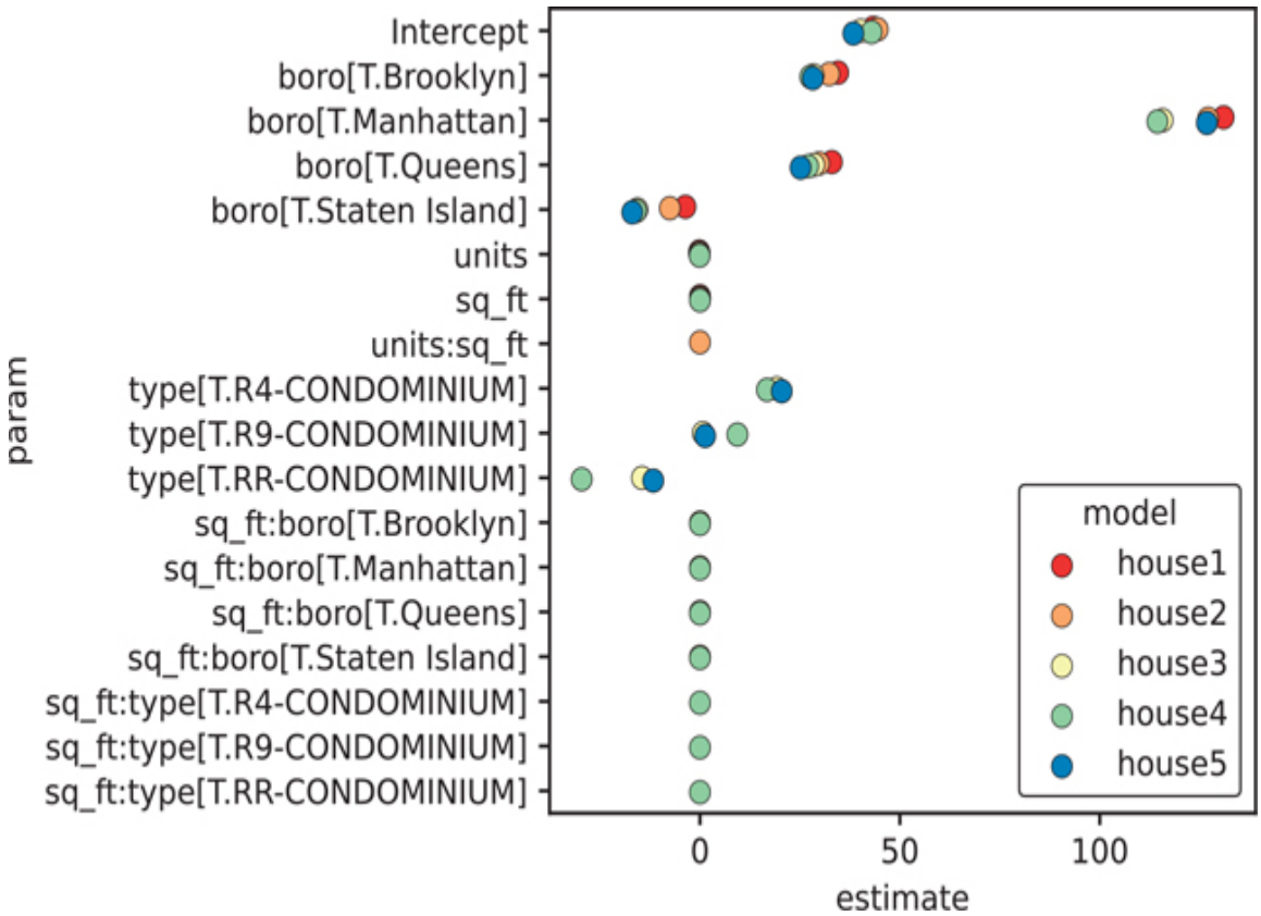
Figure 16.5 Coefficients of the house1 to house5 models
