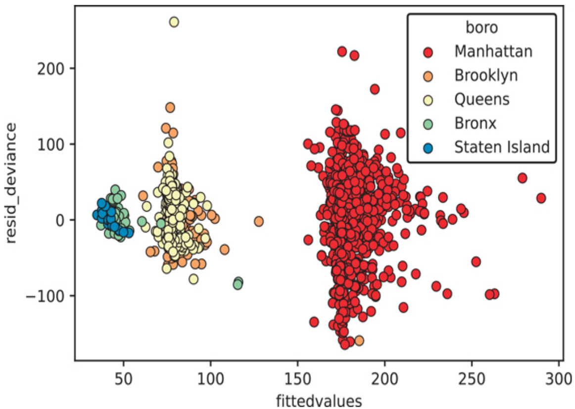
Figure 16.2 Residuals of the house1 model colored by boro
