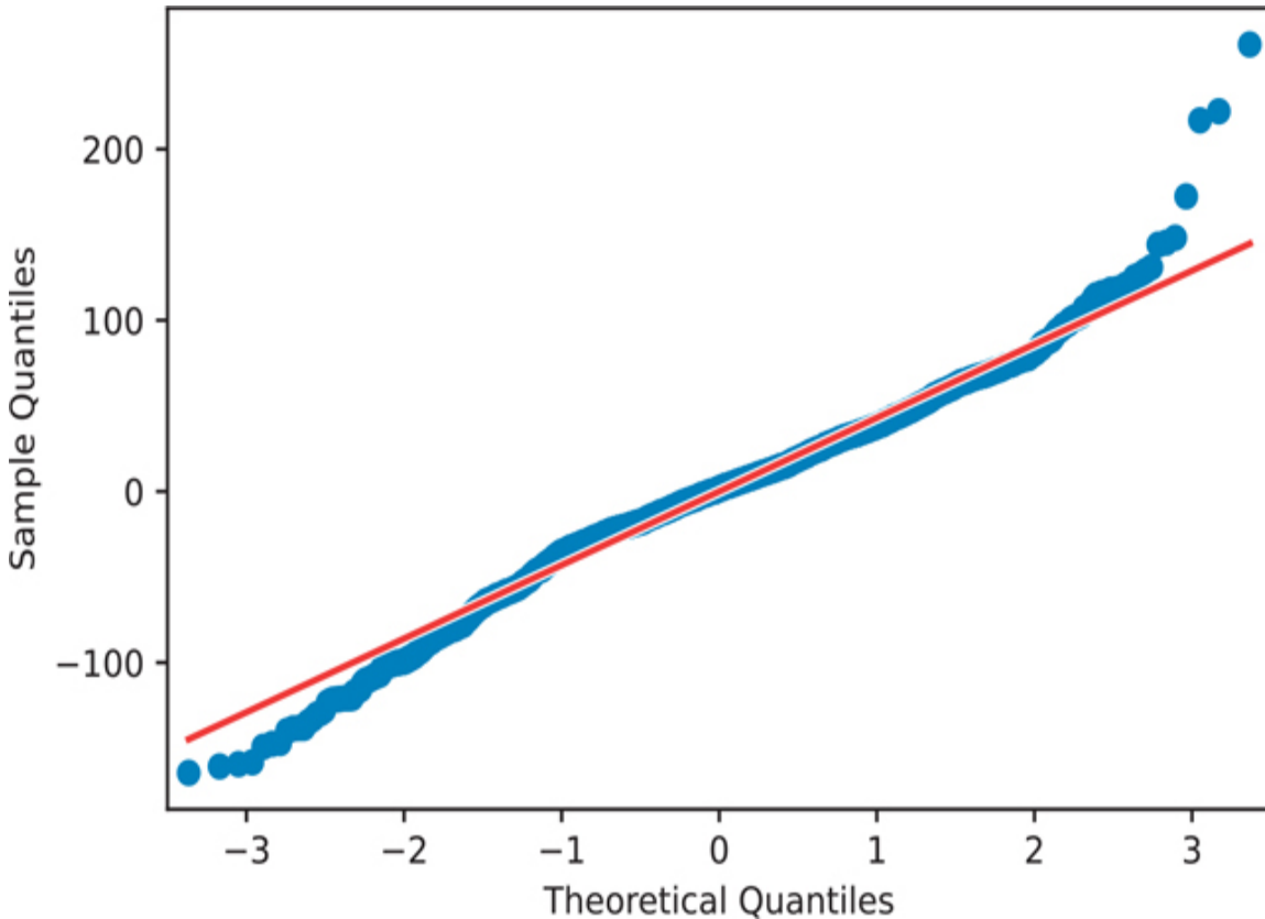
Figure 16.3 The q-q plot of the house1 model
