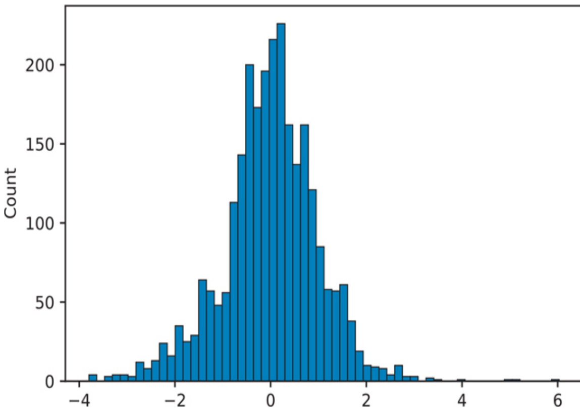
Figure 16.4 Histogram of the house1 model residuals
