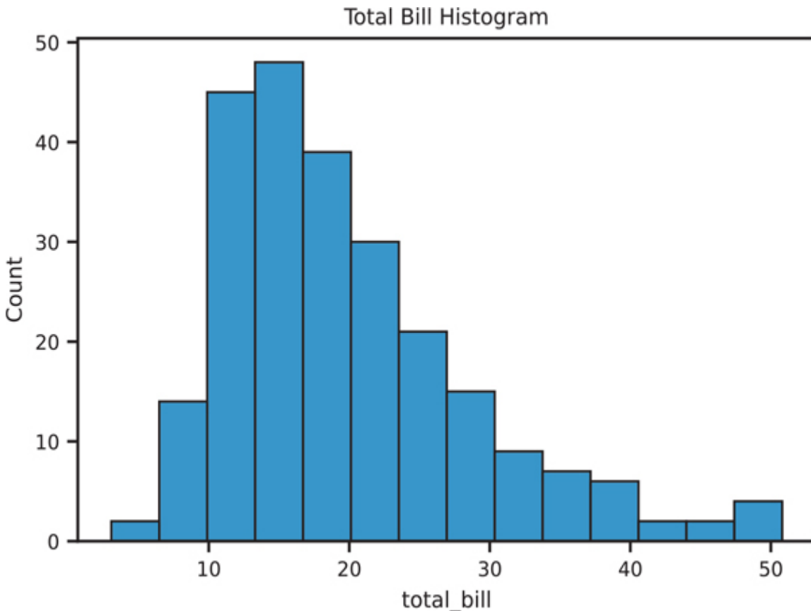
Figure 3.12 Seaborn histplot
