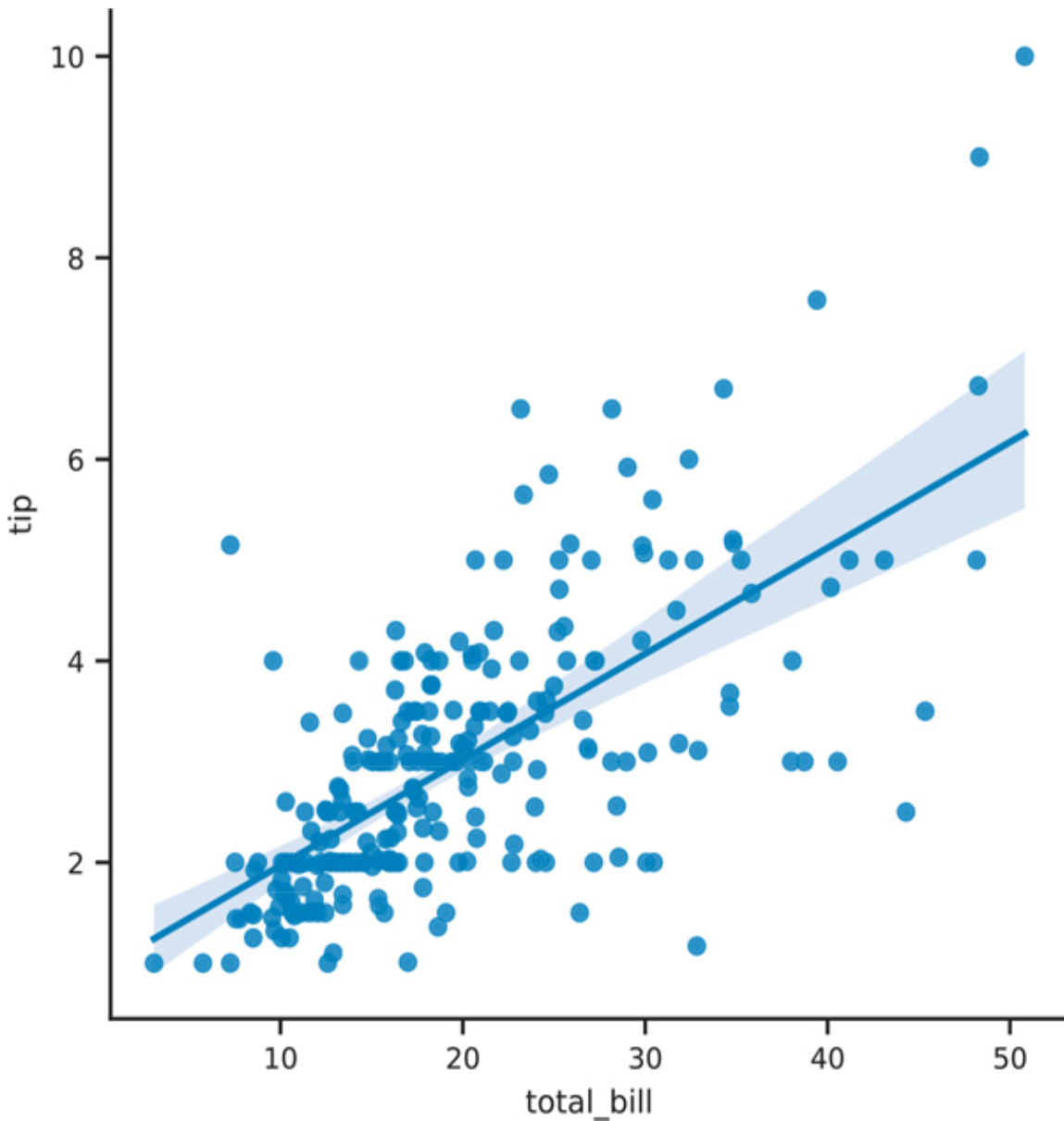
Figure 3.19 Seaborn scatter plot using sns.lmplot()
