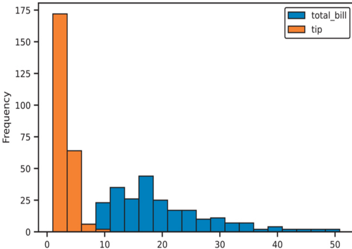
Figure 3.45 Histogram of a Pandas DataFrame
