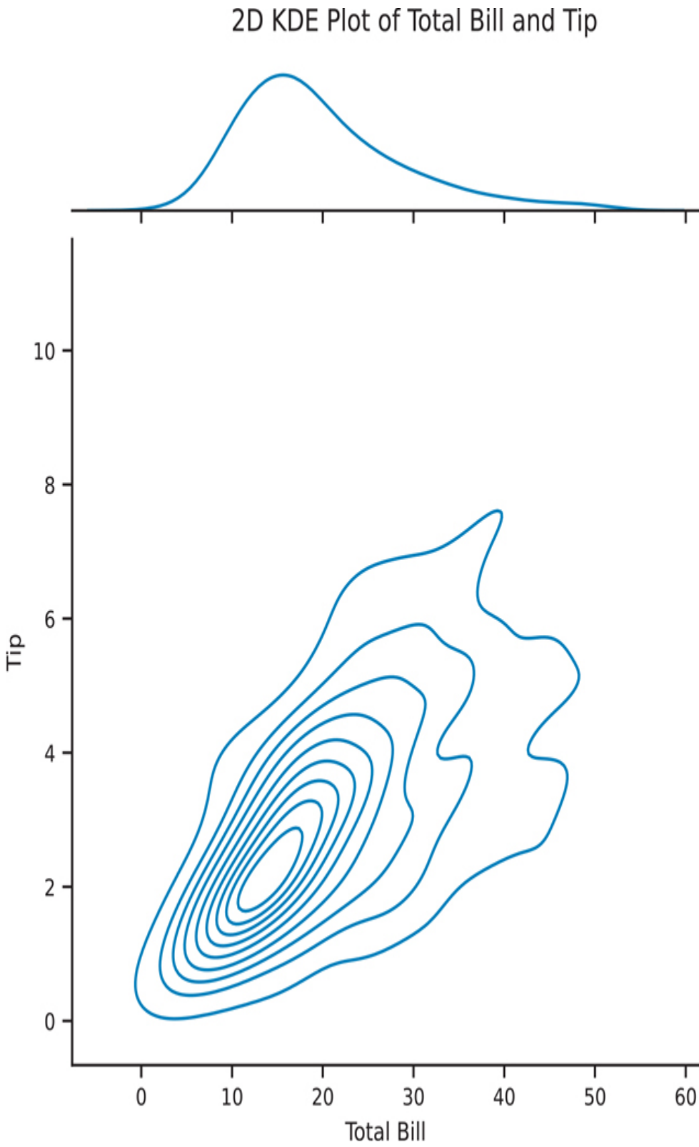
Figure 3.23 Seaborn KDE plot using sns.jointplot()
