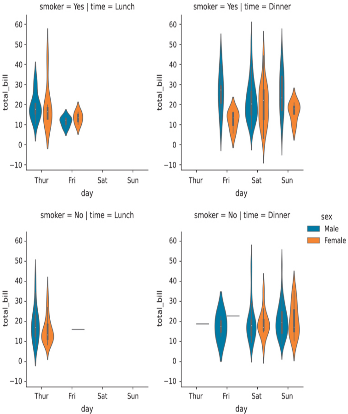
Figure 3.39 Seaborn plot with manually created facets with two non-overlapping variables
