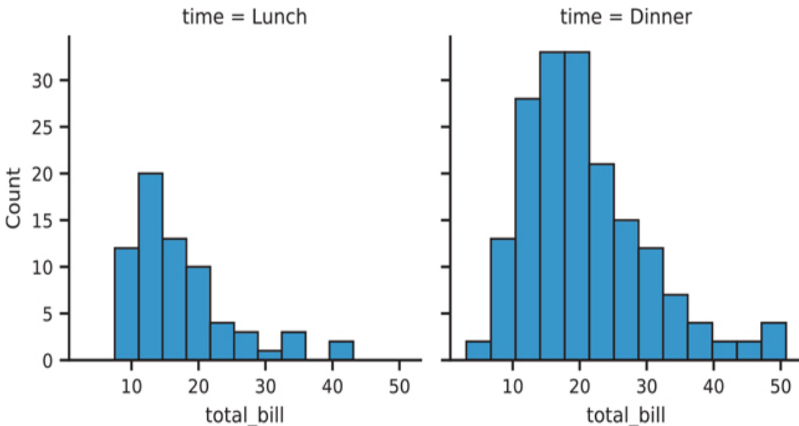
Figure 3.36 Seaborn plot with manually created facets
