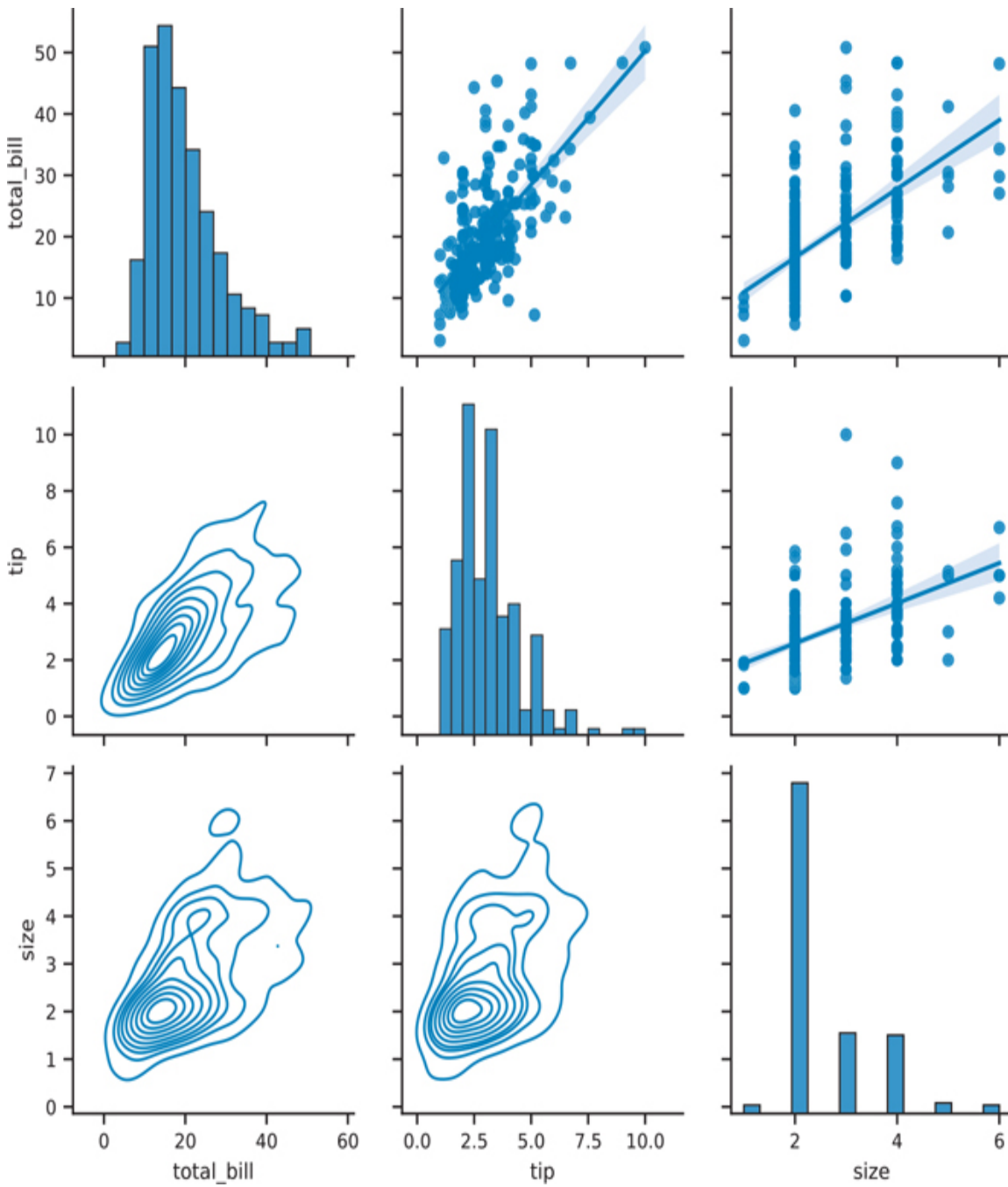
Figure 3.29 Seaborn pair plot with different plots on the upper and lower halves
