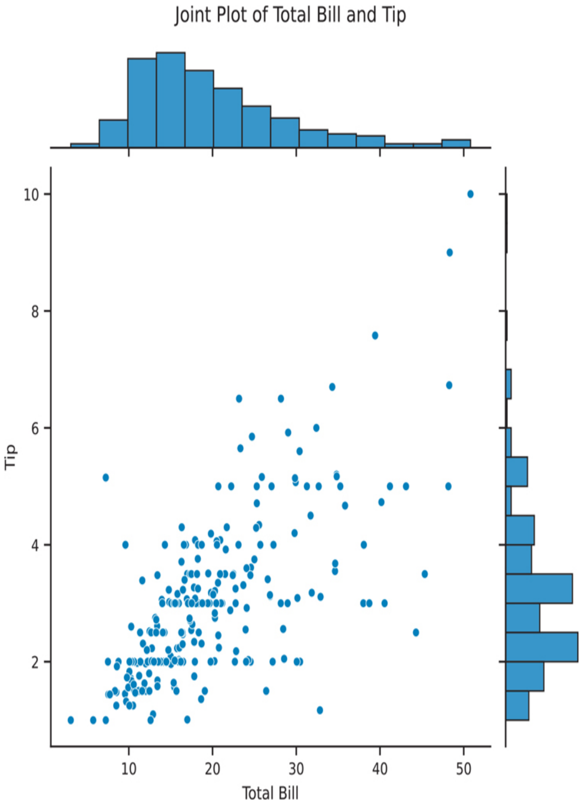
Figure 3.20 Seaborn scatter plot using sns.jointplot()
