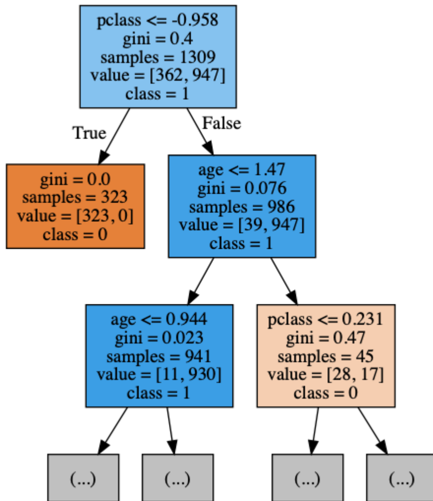
Figure 18-8. Decision tree explaining the clustering
