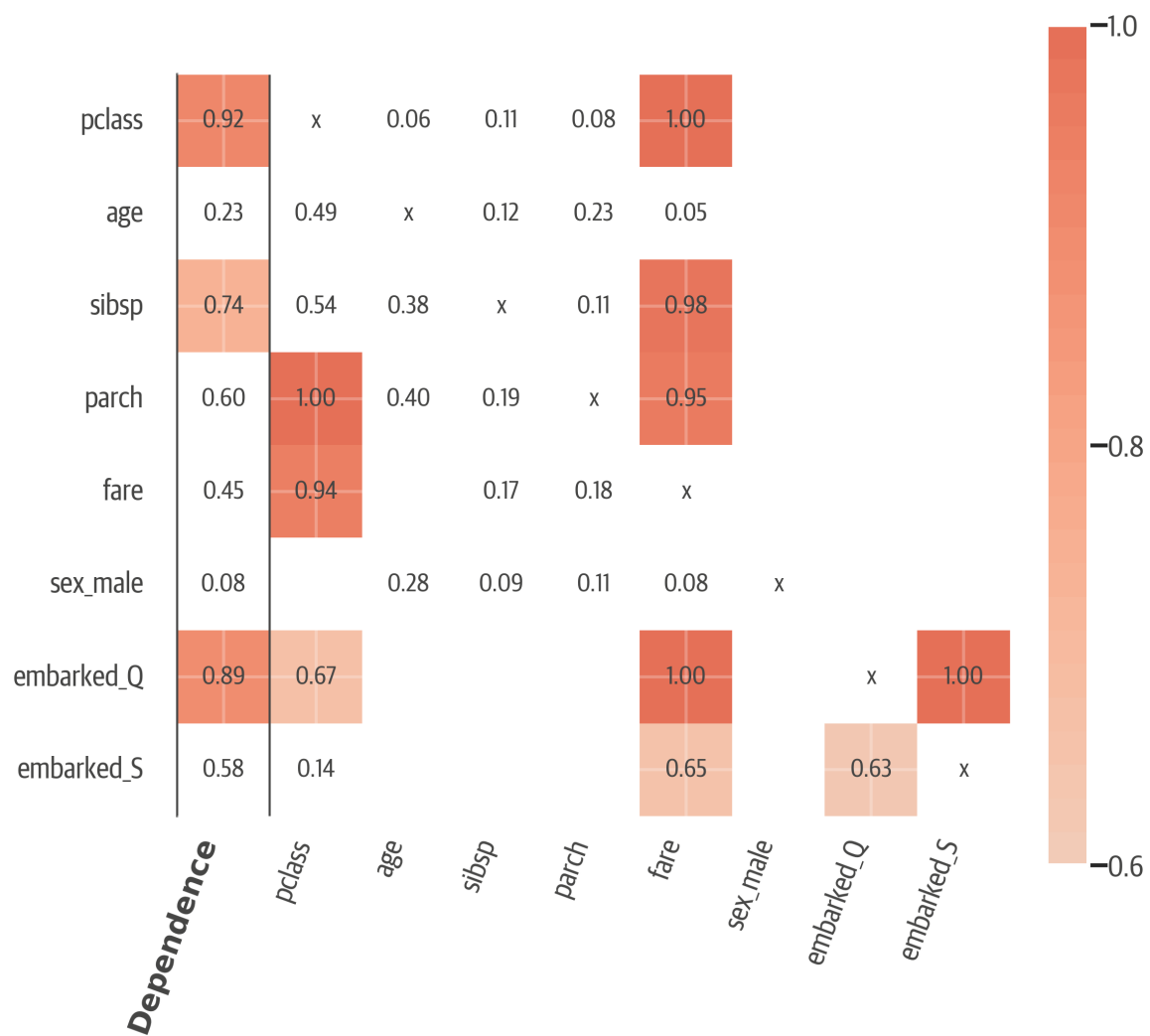
Figure 8-1. Dependence heat map. Pclass, sibsp, parch, and embarked_Q can be predicted from fare, so we can remove them.
