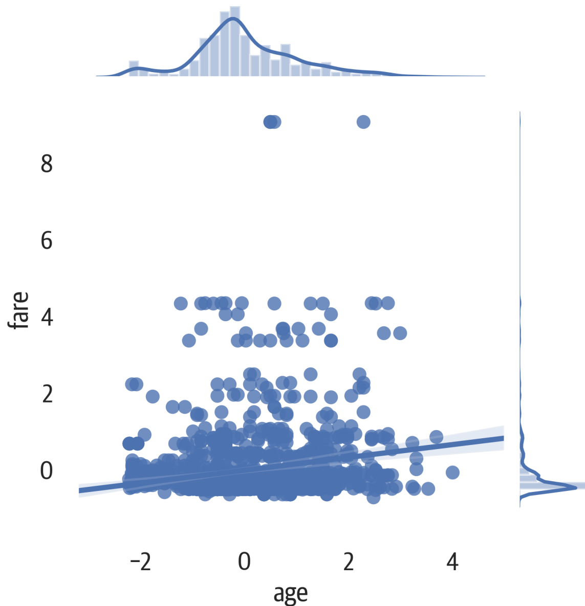
Figure 6-5. Seaborn joint plot.
