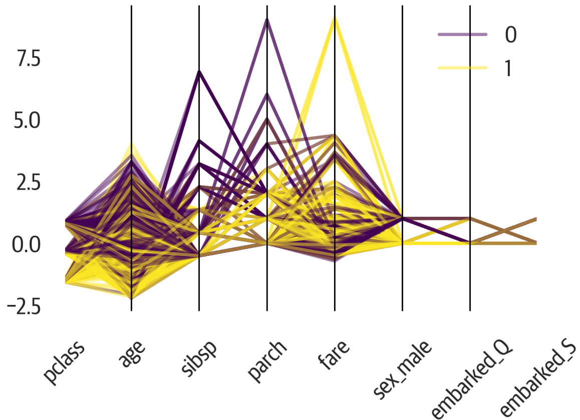
Figure 6-15. Pandas parallel coordinates plot.
