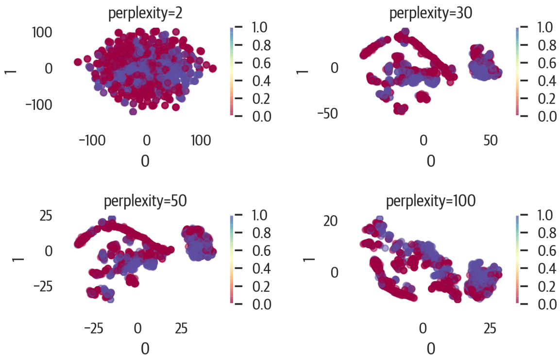
Figure 17-17. Changing perplexity for t-SNE.
