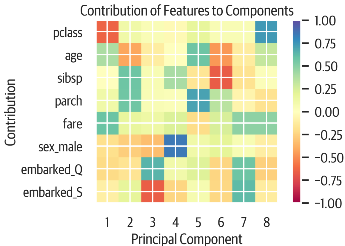
Figure 17-3. PCA features in components.
