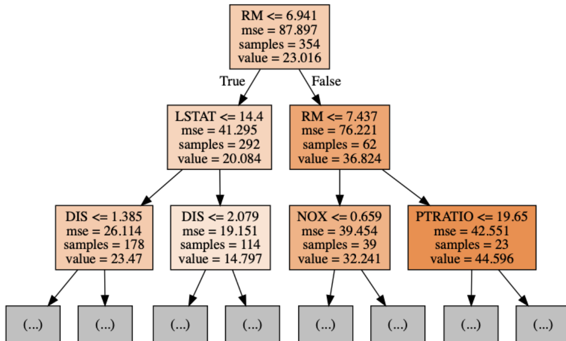
Figure 14-3. The first two layers of a decision tree.
