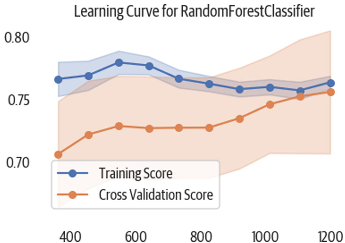
Figure 3-6. This learning curve shows that as we add more training samples, our cross-validation (testing) scores appear to improve.
