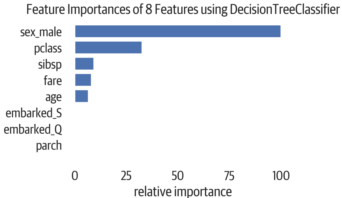
Figure 10-4. Feature importance (Gini coefficient) for decision tree (normalized to male importance).
