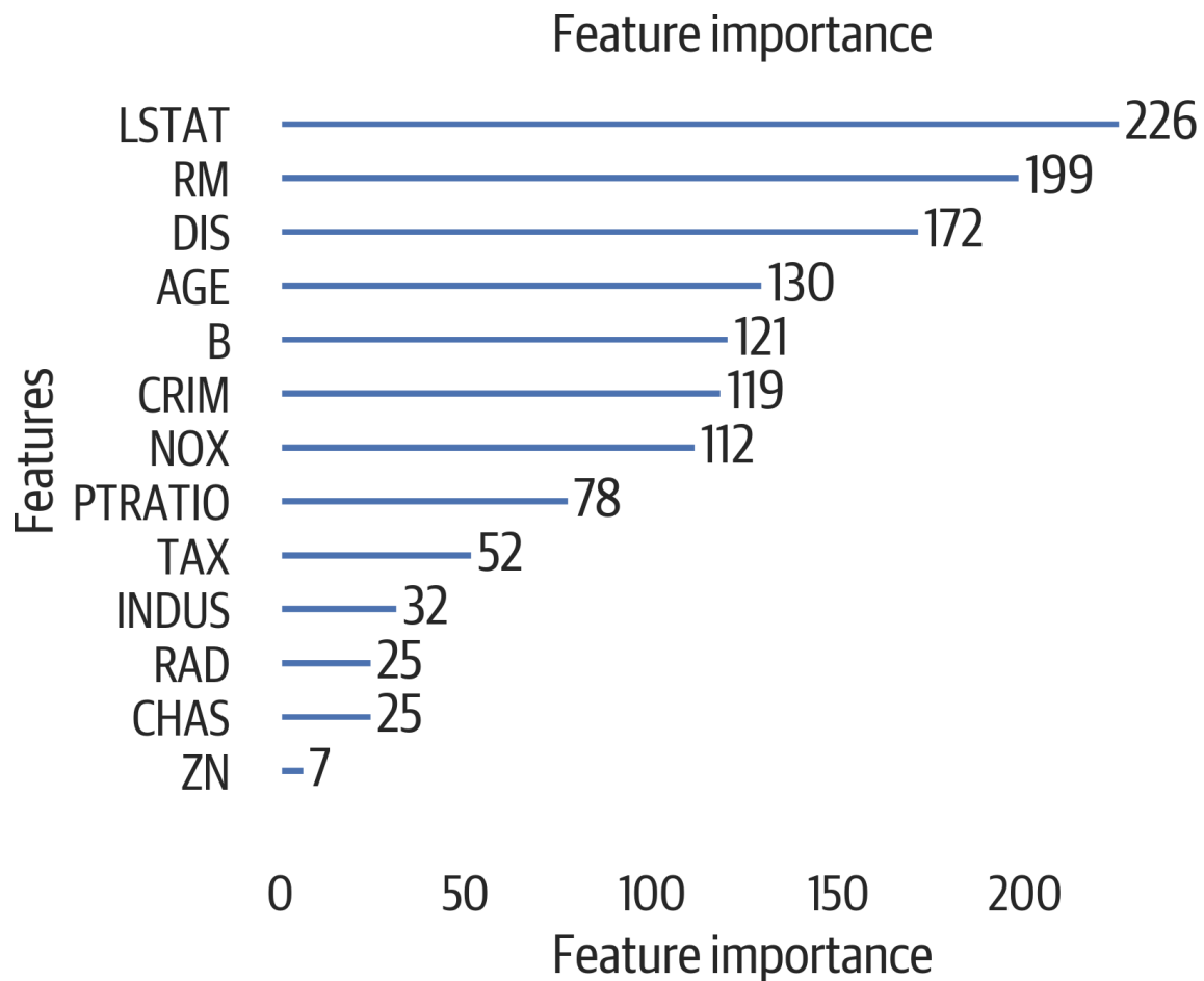
Figure 14-8. Feature importance showing how many times a feature is used.
