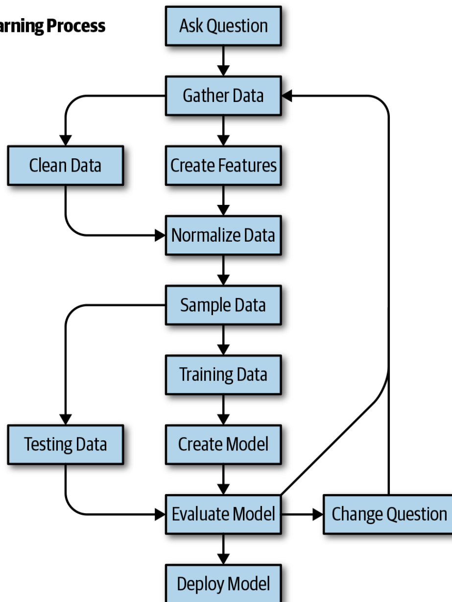
Figure 2-1. Common workflow for machine learning.
