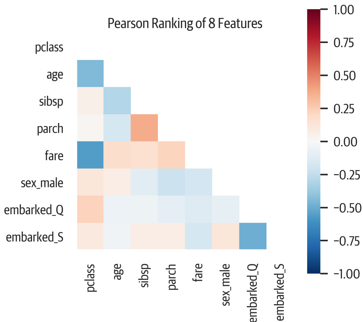
Figure 6-10. Covariance correlation created with Yellowbrick.
