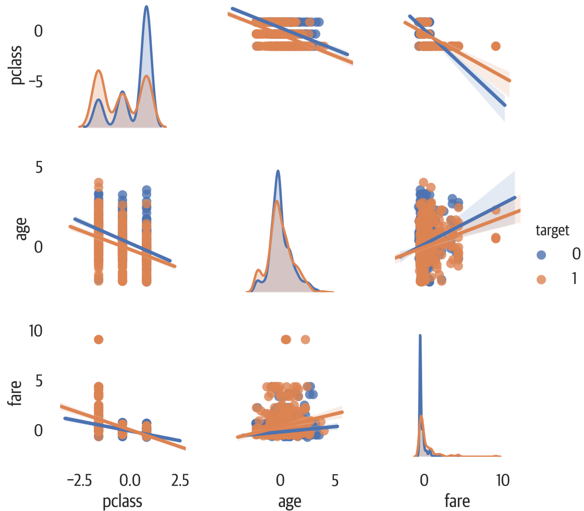
Figure 6-6. Seaborn pair grid.
