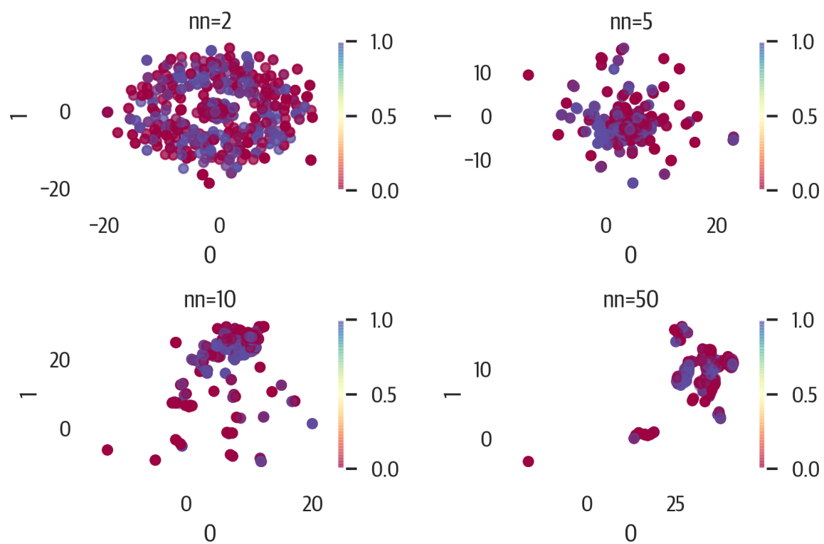
Figure 17-14. UMAP results adjusting n_neighbors .
