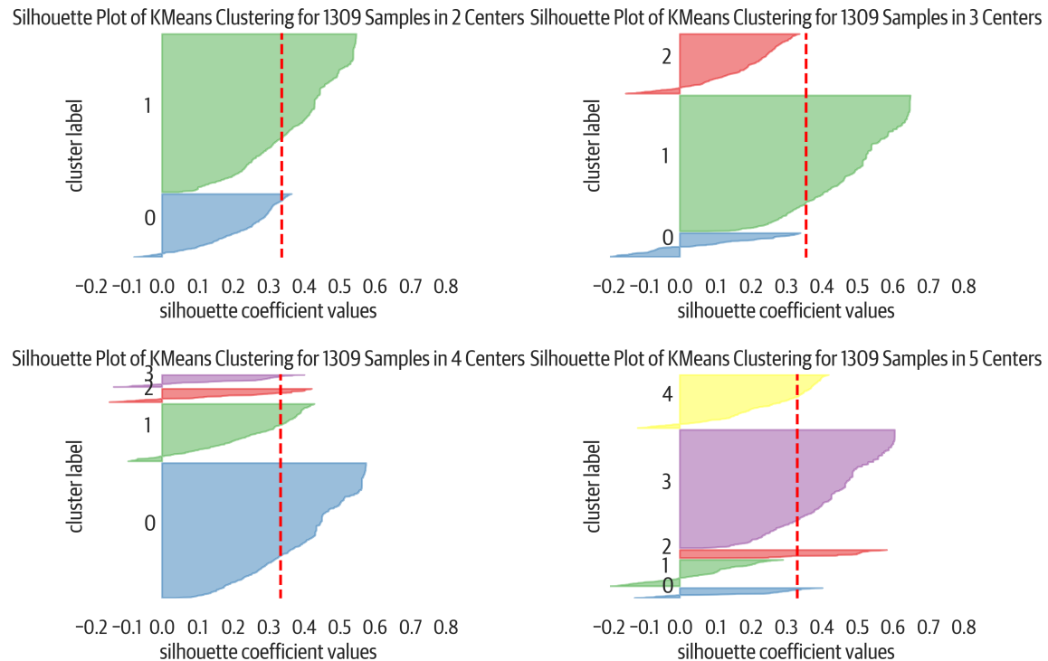
Figure 18-3. Yellowbrick silhouette visualizer
