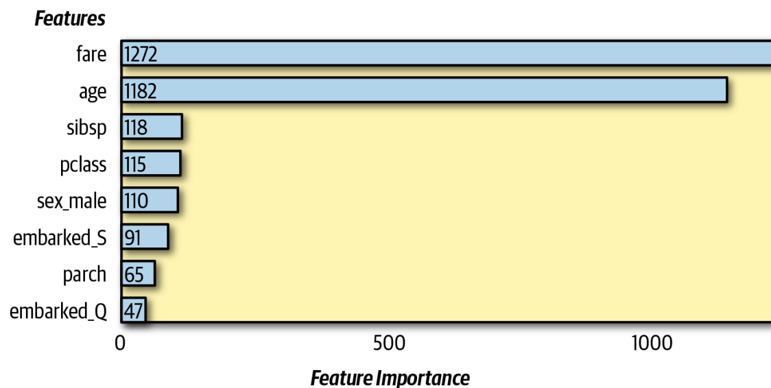
Figure 10-8. Feature importance splits for LightGBM.
