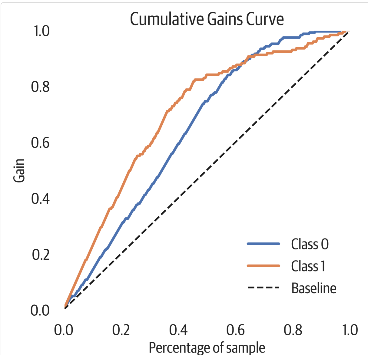
Figure 12-6. Cumulative gains plot. If we ordered people on the Titanic according to our model, looking at 20% of them we would get 40% of the survivors.
