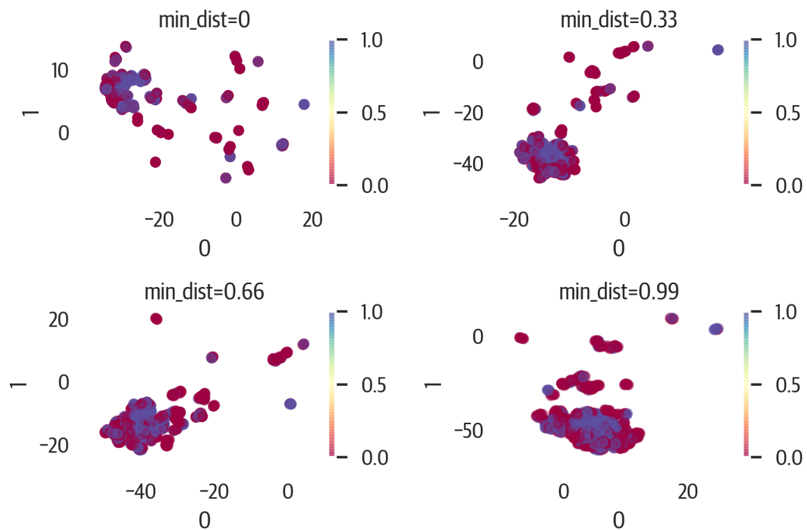
Figure 17-15. UMAP results adjusting min_dist .
