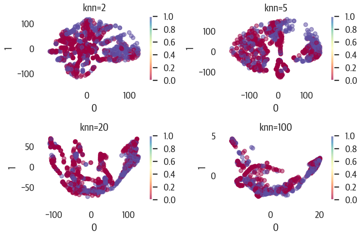
Figure 17-19. Changing the knn parameter for PHATE.
