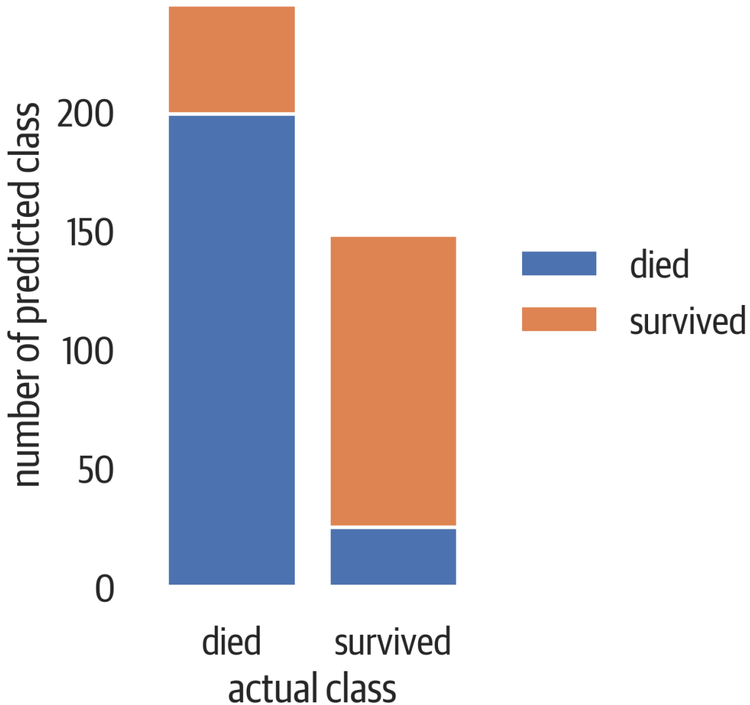
Figure 12-9. Class prediction error. At the top of the left bar are people who died, but we predicted that they survived (false positive). At the bottom of the right bar are people who survived, but the model predicted death (false negative).
