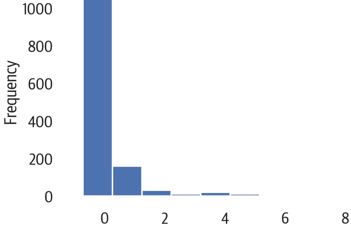
Figure 6-1. Pandas histogram.
