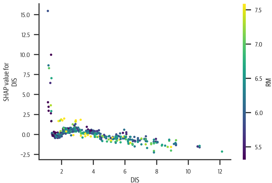
Figure 16-4. Dependence plot for DIS. Unless DIS is very small, SHAP stays relatively flat.
