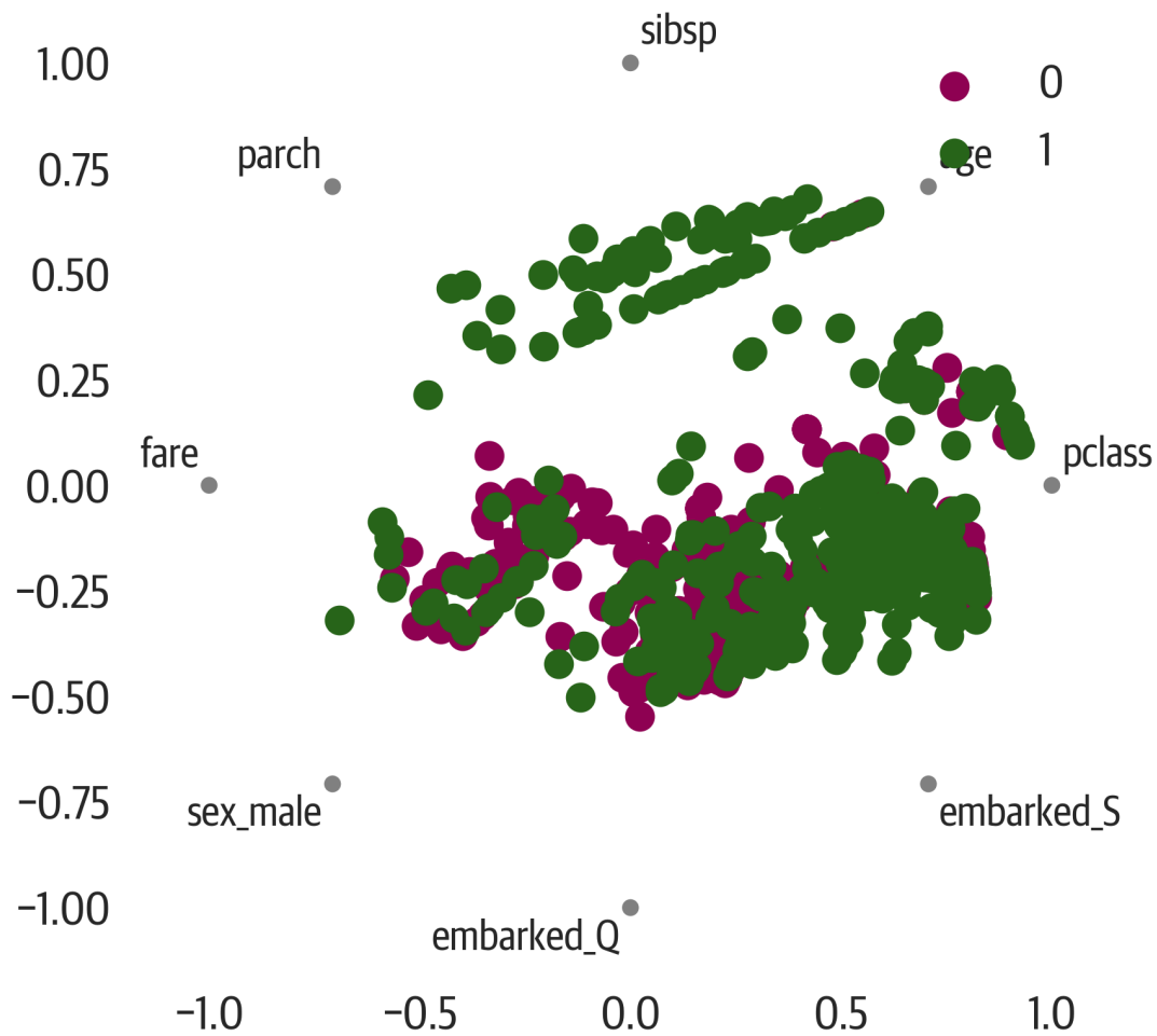
Figure 6-13. Pandas RadViz plot.
