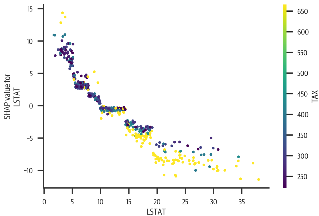
Figure 16-3. Dependence plot for LSTAT. As LSTAT goes up, the predicted value goes down.
