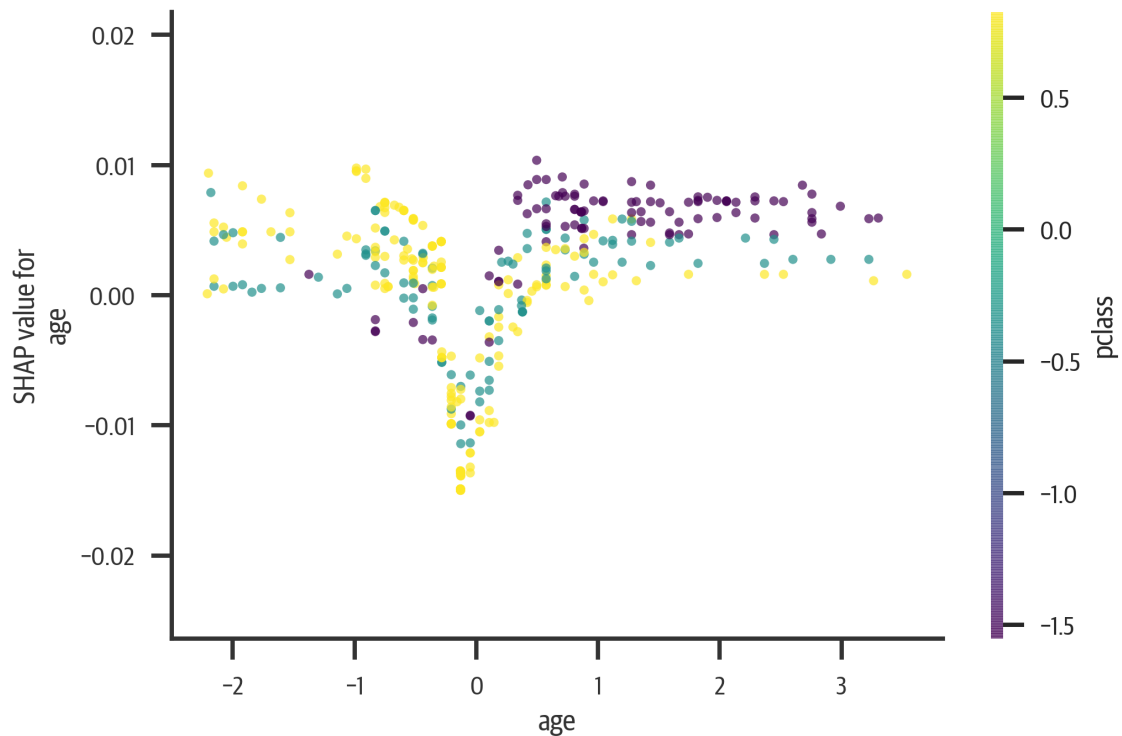
Figure 13-6. Shapley dependency plot for age. Young and old have a higher rate of survival. As age goes up, a lower pclass has more chance of survival.
