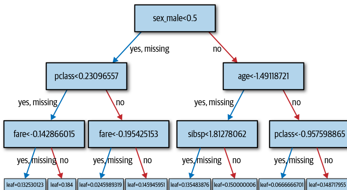
Figure 10-7. Tree of XGBoost.
