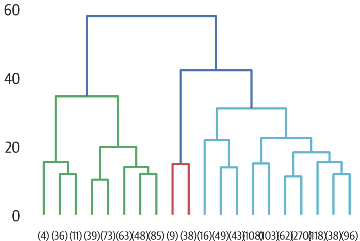
Figure 18-5. Truncated hierarchical clustering dendrogram. If we cut across the largest vertical lines, we get three clusters.
