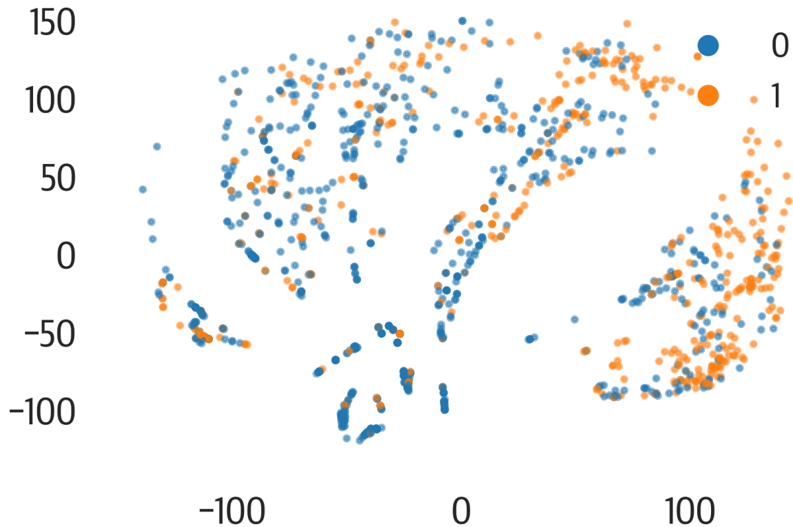
Figure 17-18. PHATE results.
