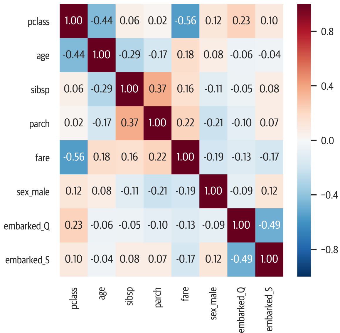
Figure 6-11. Seaborn heat map.
